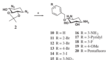
Scheme 2. Reagents and conditions: (a) i: RCH 2 Br, DMF, NaH; ii: CH 3 CO 2 H/H 2 O, 60 °C, 3 h; iii: Me 3 P/THF/H 2 O, 35–55% overall yields.
